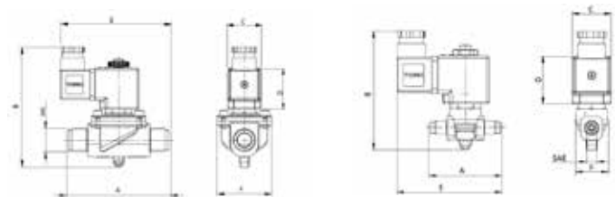
Pilot Operated Dimensions (mm)
