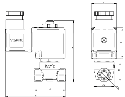
Dimensions (mm)
