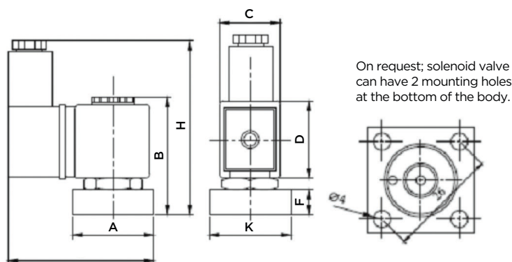
Dimensions (mm)
