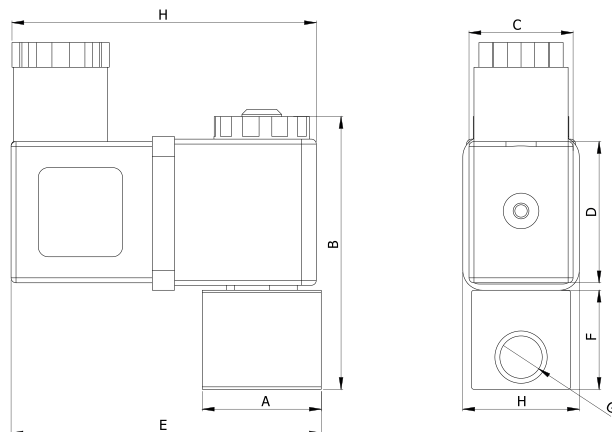
Dimensions (mm)
