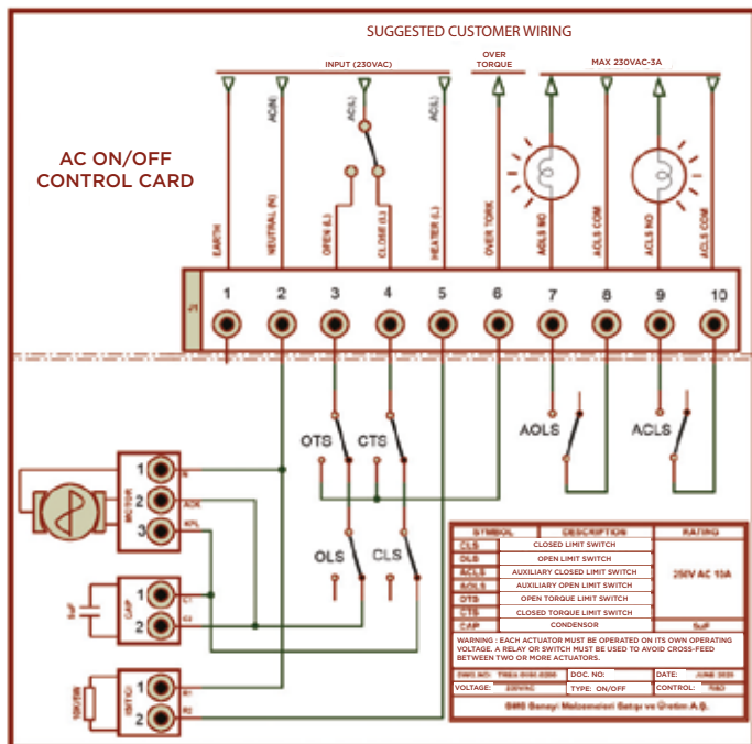
Figure 20: 230V AC ON/OFF Electric Actuator Connection Diagram
