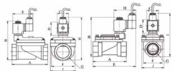
Dimensions (mm)
