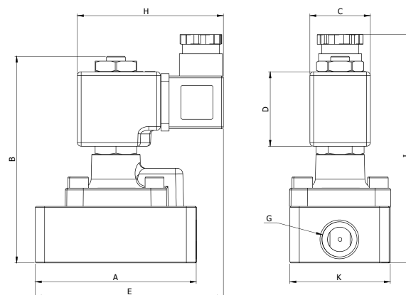
Dimensions (mm)
