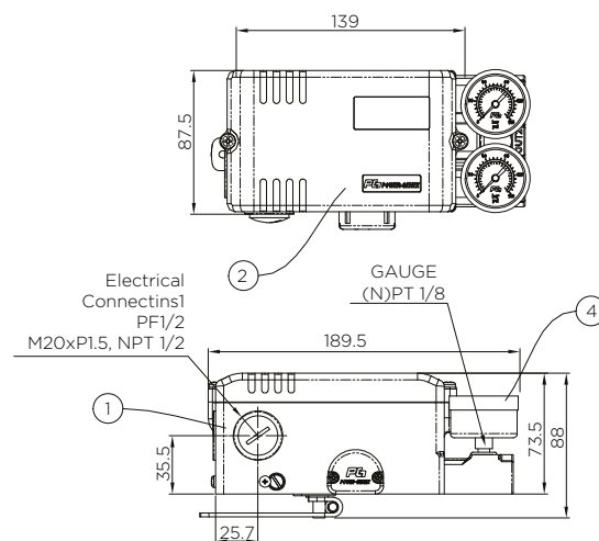
TORK-EPR Electromechanic Positioner (Rotary) TORK-EPL Electromechanic Positioner (Linear)
