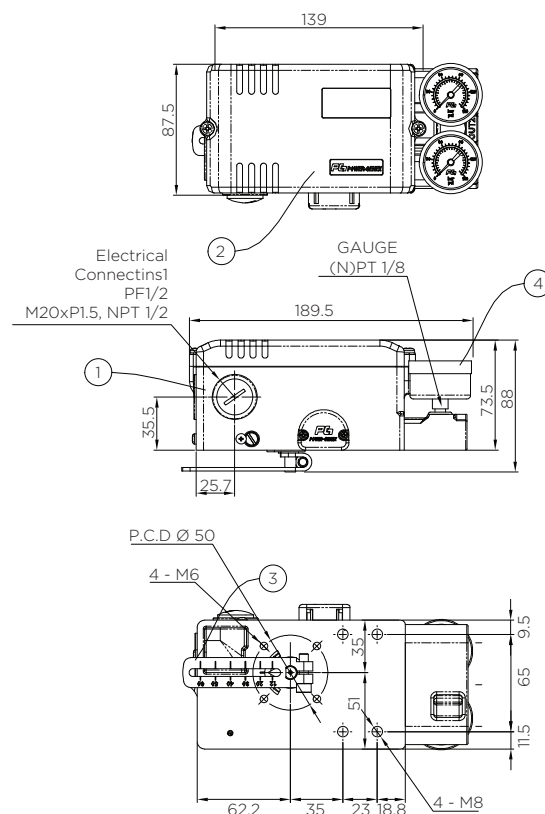
TORK-EPR Electro - Pneumatic Positioner
