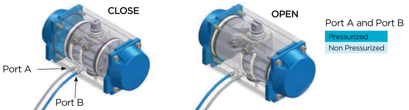
Fig 2. Double Acting Actuators
