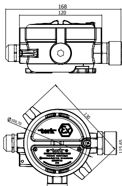
Figure 5: Technical Dimensions
