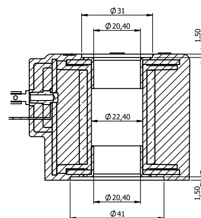
SECTION M-M
